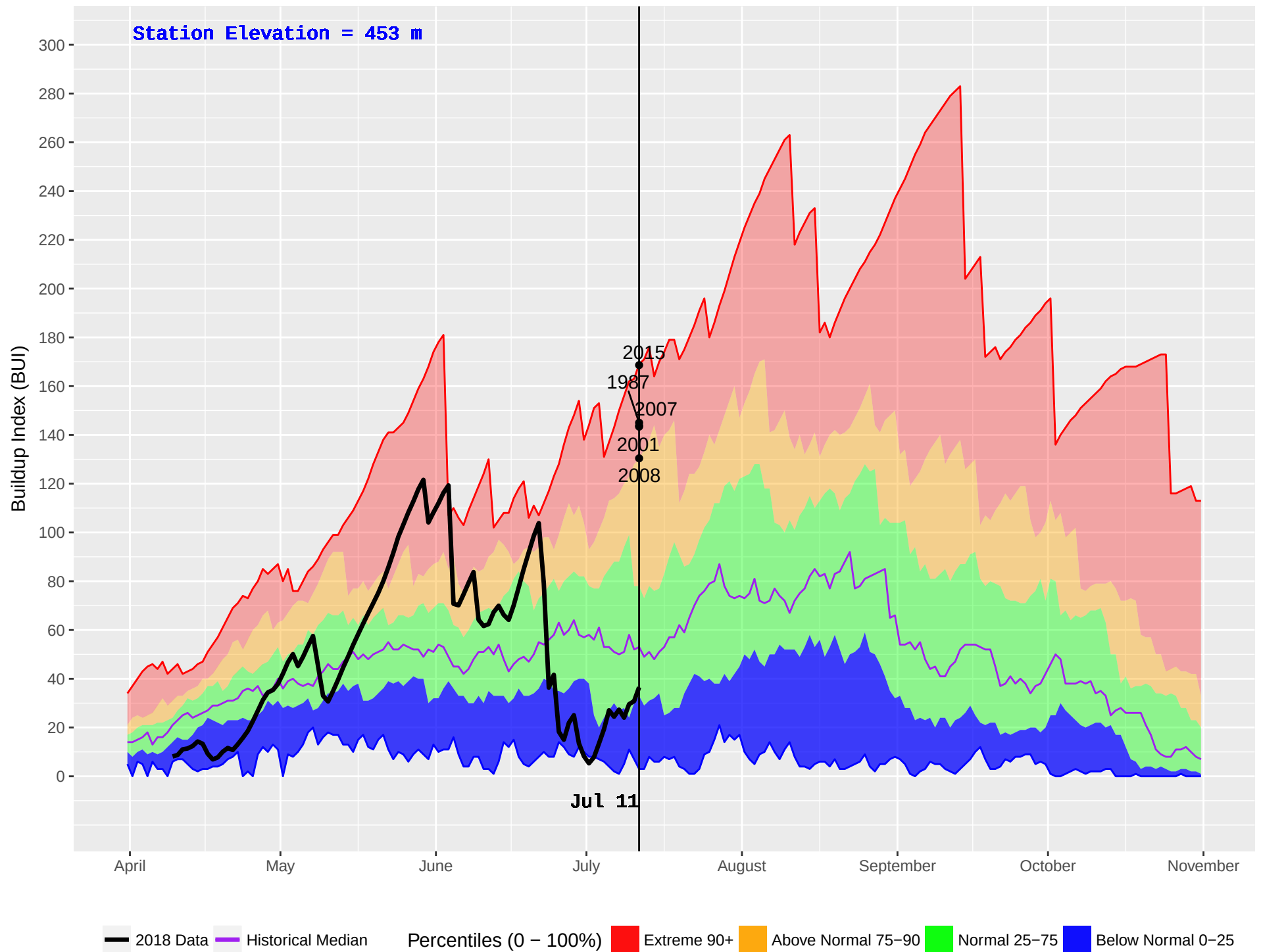
CLEARWATER HUB (239) : Historical (1976–2016) and Current (2018) Noon Buildup Index (BUI)
